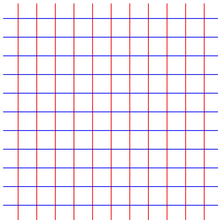
Figure 1: Standard grid in the complex plane
