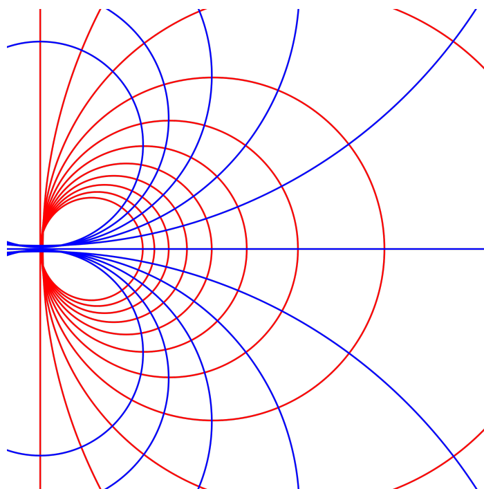
Figure 2: The same grid after applying the function z \mapsto \frac{1}{z} (which is the Möbius transformation given by \begin{pmatrix} 0 & 1 \\ 1 & 0 \end{pmatrix} )
