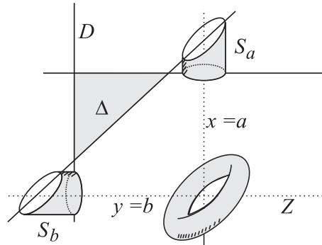
Fig. 15.4 Generators of H_2^{\text{sing}}(X, D; \mathbb{Q})
